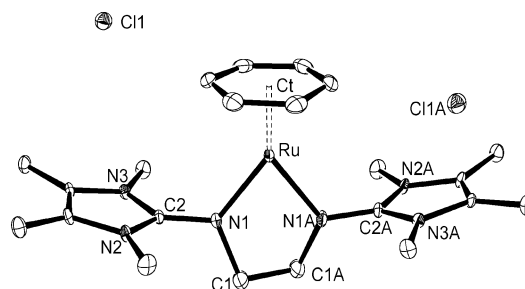
Figure 2. ORTEP diagram of [(\eta^6\text{-C}_6\text{H}_6)\text{Ru}(\text{BL}^{\text{Me}})]\text{Cl}_2 ( [5]Cl ) with thermal displacement parameters drawn at 50% probability. The letter "A" indicates atoms generated via the twofold axis.
