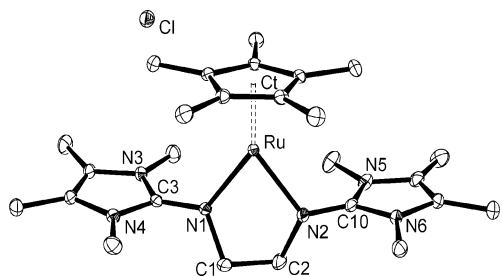
Figure 1. ORTEP diagram of the complex [3]Cl with thermal displacement parameters drawn at 50% probability.
