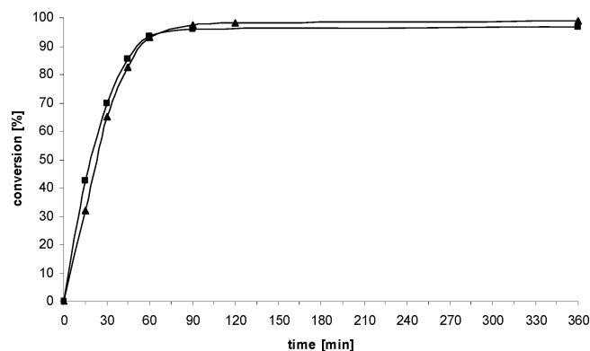
Figure 6. Conversion/time diagrams for [3]Cl (squares) and [3]BAr F (triangles).
