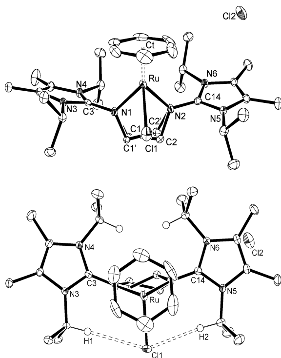
Figure 3. Two ORTEP diagrams of [(\eta^6\text{-C}_6\text{H}_6)\text{Ru}(\text{BL}^{\text{Pr}})\text{Cl}]\text{Cl} in [\text{6}]\text{Cl}_2\cdot\text{thf} with thermal displacement parameters drawn at 50% probability; the ethylene bridge is disordered.
