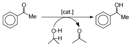
Scheme 5. Transfer hydrogenation of acetophenone.
