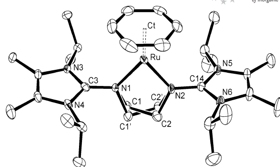
Figure 4. ORTEP diagram of the cation in [\text{6}](\text{BF}_4)_2\cdot\text{CH}_2\text{Cl}_2 with thermal displacement parameters drawn at 50% probability; the ethylene bridge is disordered.
