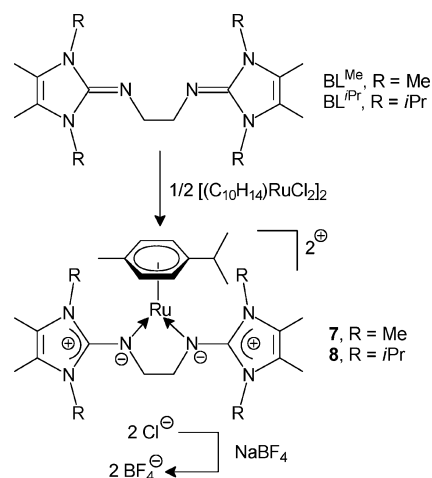
Scheme 4. Synthesis of [7] and [8].
