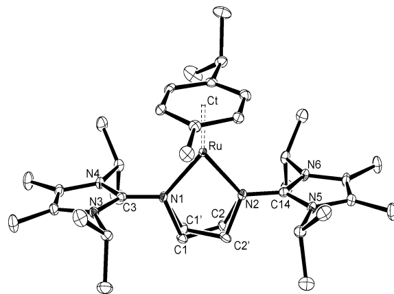
Figure 5. ORTEP diagram of the cation in [\text{8}](\text{BF}_4)_2\cdot\text{CH}_2\text{Cl}_2 with thermal displacement parameters drawn at 50% probability; the ethylene bridge is disordered.
